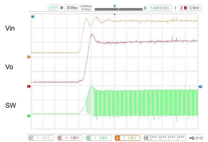
6. Start-up Waveform
