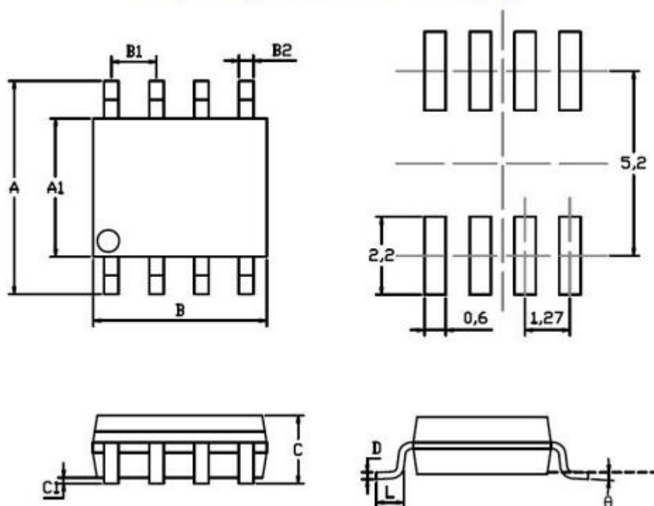
SOP8 package mechanical drawing
