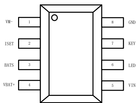
SOP-8L (Top View)
