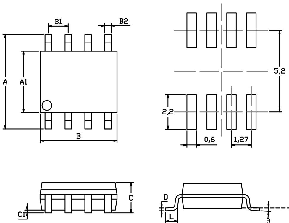
SOP8 package mechanical drawing
