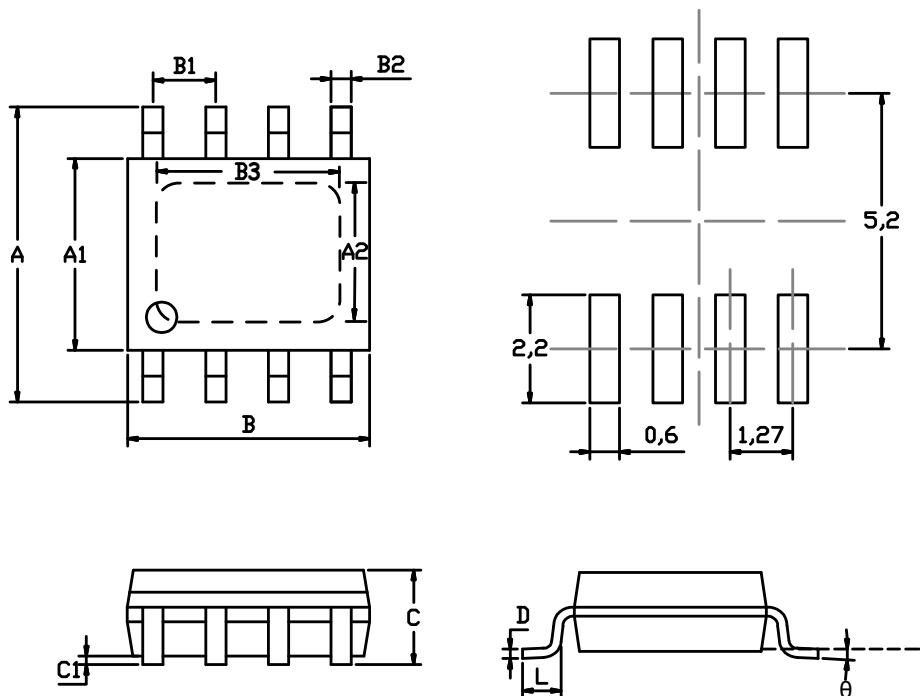
ESOP8 package mechanical drawVCCg
