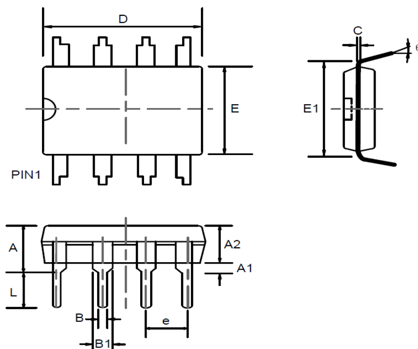
DIP8 package mechanical drawing
